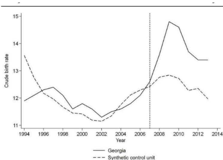
Fig. 5 Crude birth rate per 1000 comparison between Georgia and its synthetic control unit. Note: covariate balance, weights of countries in the synthetic control unit (Armenia, Azerbaijan, Estonia, and Romania), and estimated size of the impact are provided in Tables A.5, A.6, and A.7
