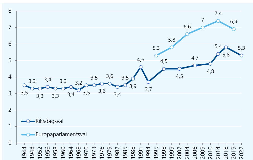
Figur 4 Det svenska partisystemets fragmenteringsgrad i samband med riksdagsval och Europaparlamentsval 1944–2022 (effektivt antal partier). Party system fragmentation in Swedish general elections and European parliamentary elections 1944–2022 (effective number of parties).
